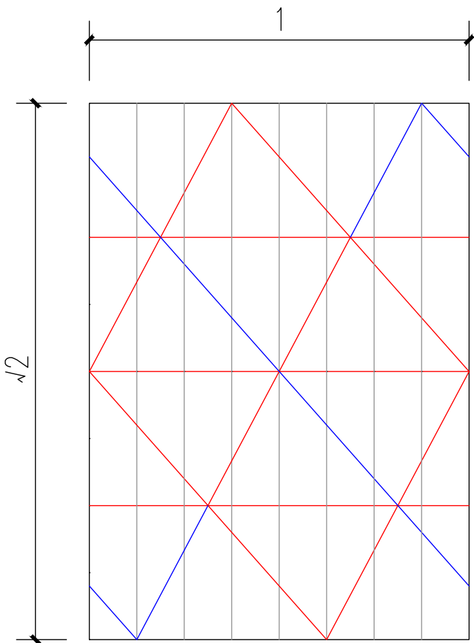
Twisted tetrahedral outer membrane 2 crease pattern (outer)
