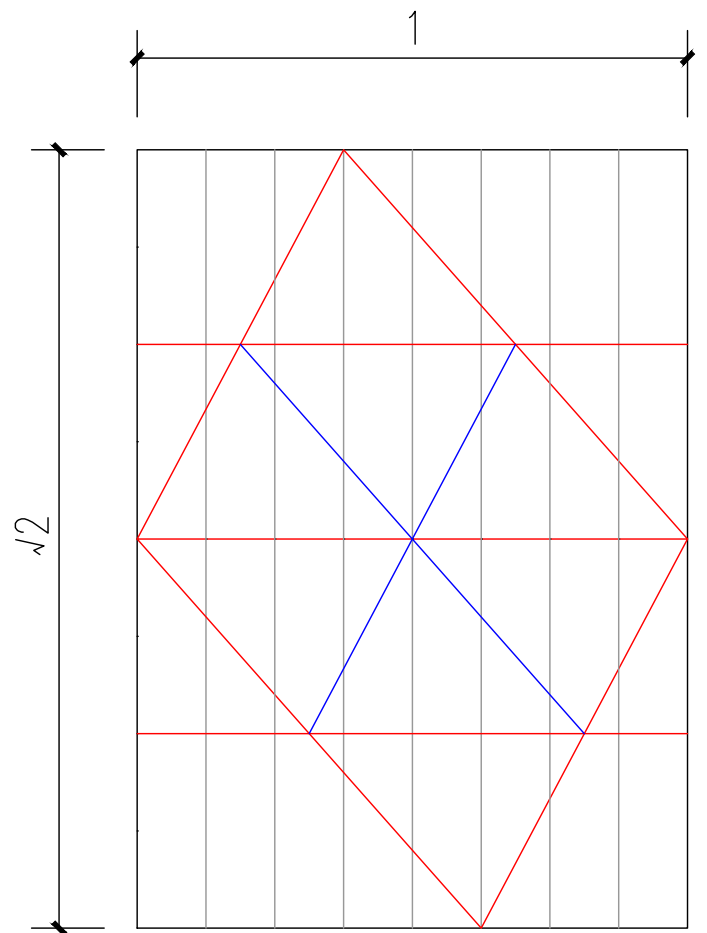
Twisted tetrahedral inner tube 2 crease pattern (outer)
