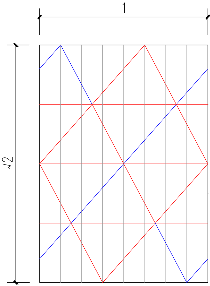
Twisted tetrahedral outer membrane 1 crease pattern (outer)
