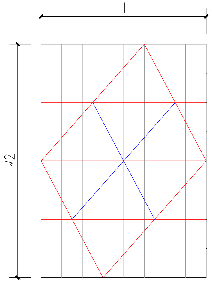
Twisted tetrahedral inner tube 1 crease pattern (outer)
